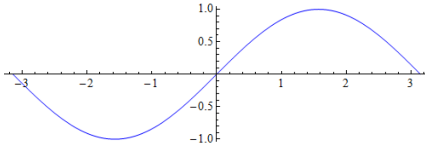
Figure 1.1: Sine function
